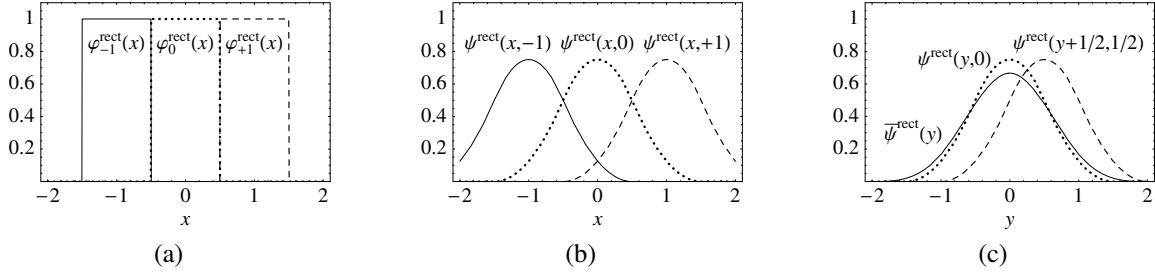
Figure 2: Response functions for the 2-tap box analysis filter \frac{1}{2}(1\ 1) .
