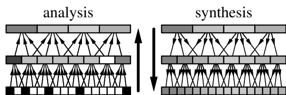
Figure 1: Illustration of pyramidal blurring in 1D.
